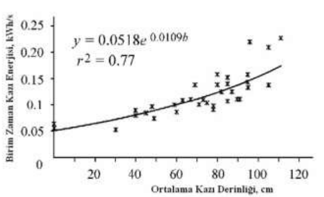
Figure 1. Depth-energy relationship.
